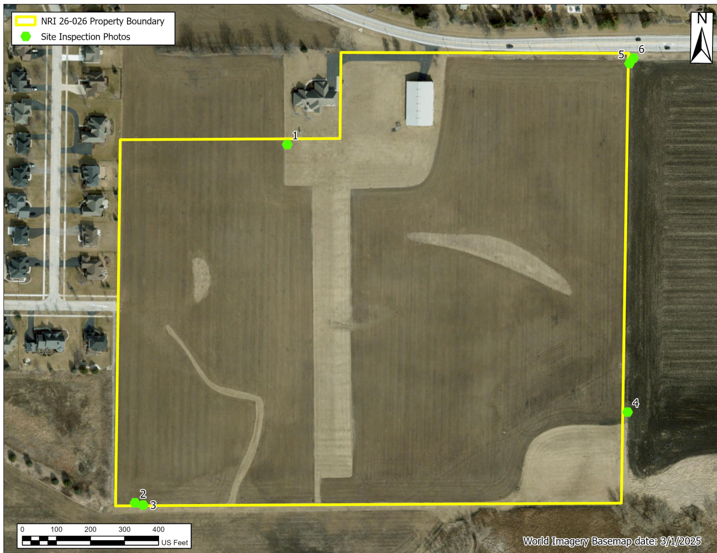
Figure 19: Location of site inspection photos
