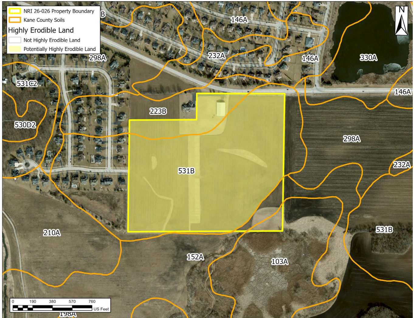
Figure 11: Highly Erodible Land map
